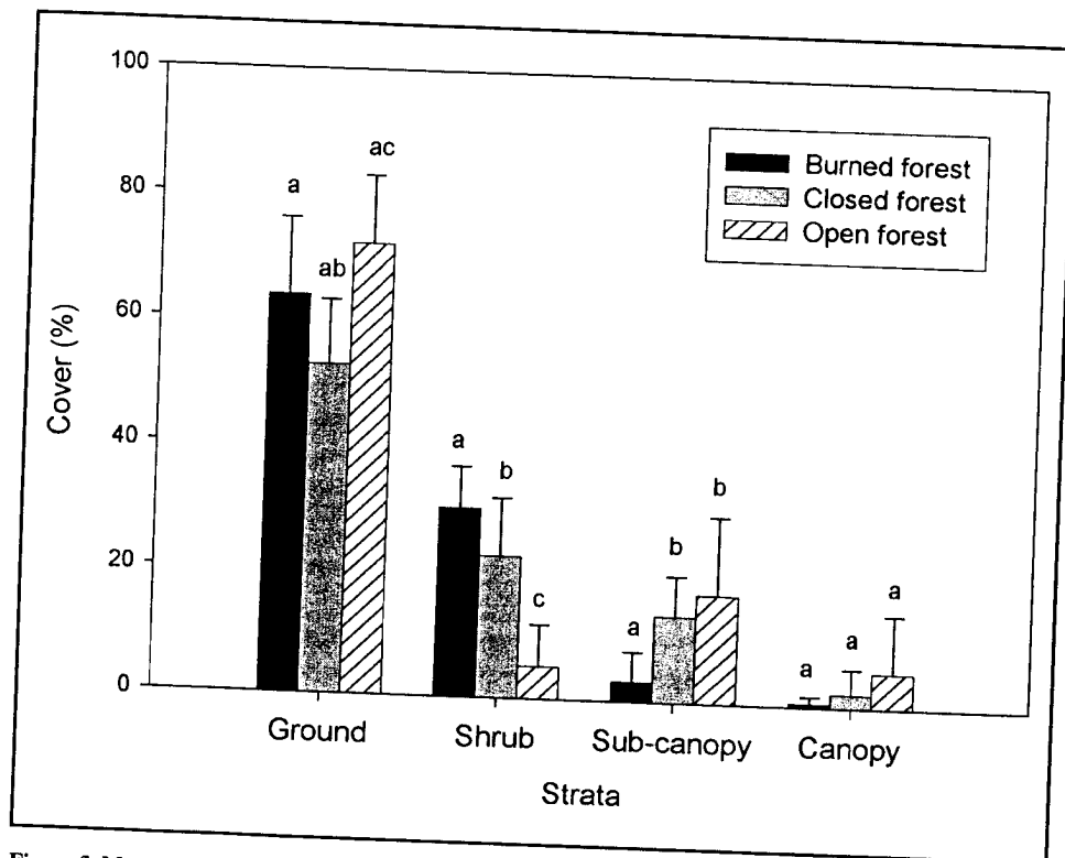
Figure 3. Mean horizontal coverage (and 1 S.D. indicated by vertical line) of the four strata in the burned, closed, and open calden forests in Parque Luro Reserve, La Pampa, Argentina. Means with the same letter indicate non-significant differences at P = 0.05 (Mann-Whitney U tests).
