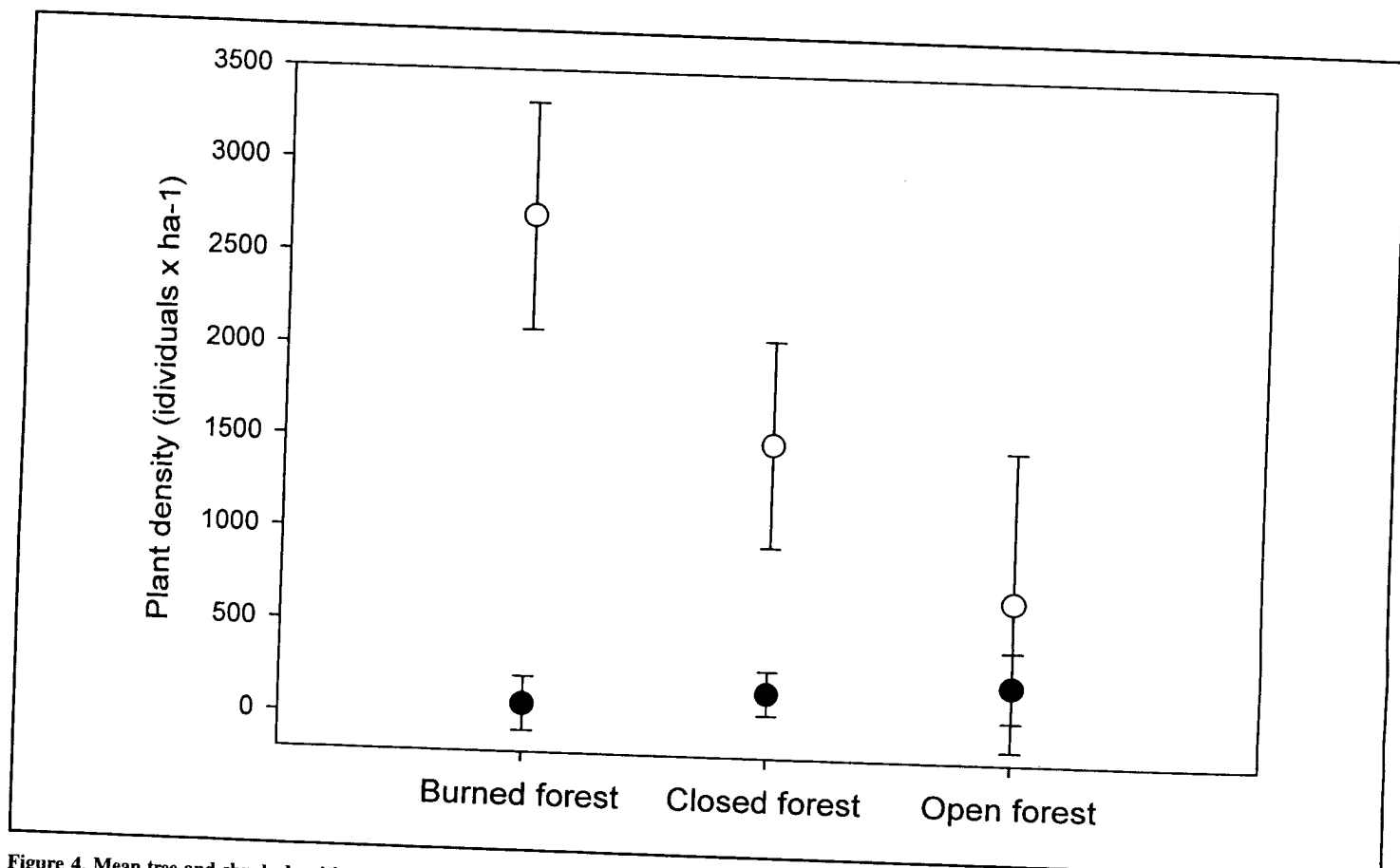
Figure 4. Mean tree and shrub densities ( \pm S.D.) in the three areas of calden forests in Parque Luro Reserve. Open circles are shrub/sapling densities and solid circles are tree densities.
